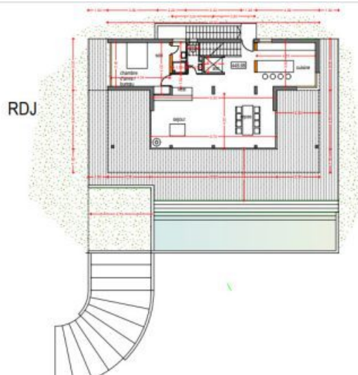
RDJ villa 1/100
