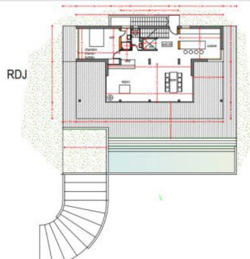
RDJ villa 1/100
