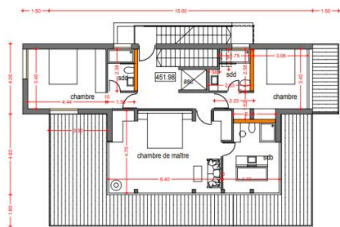
R+1 villa
