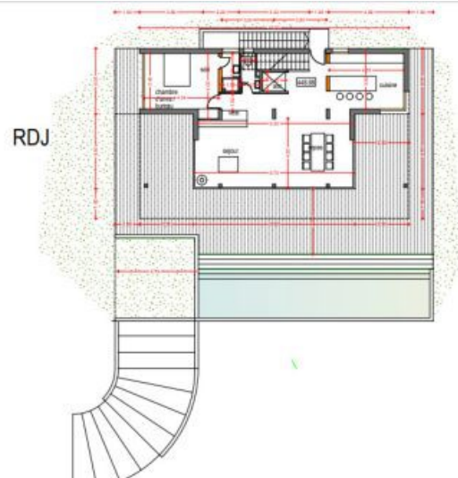
RDJ villa 1/100
